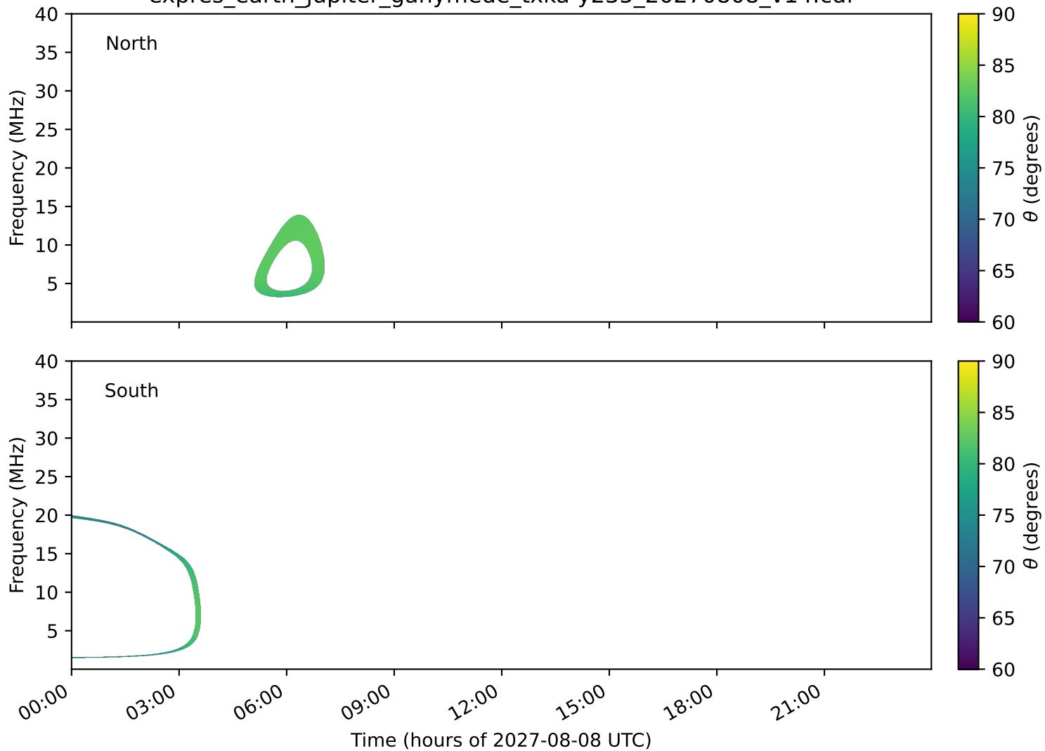
expres_earth_jupiter_ganymede_txka-y235_20270808_v14.cdf
