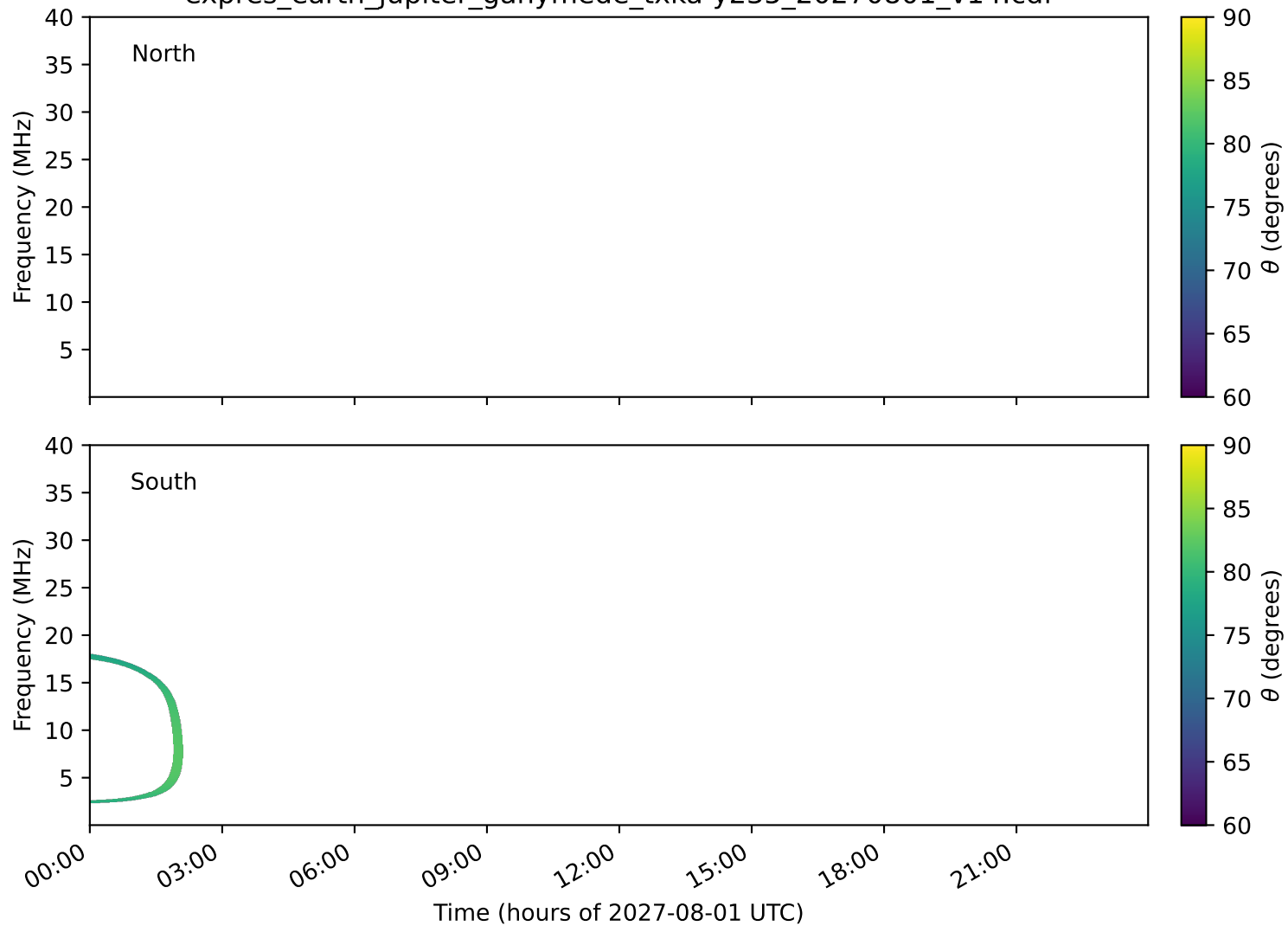
expres_earth_jupiter_ganymede_txka-y235_20270801_v14.cdf
