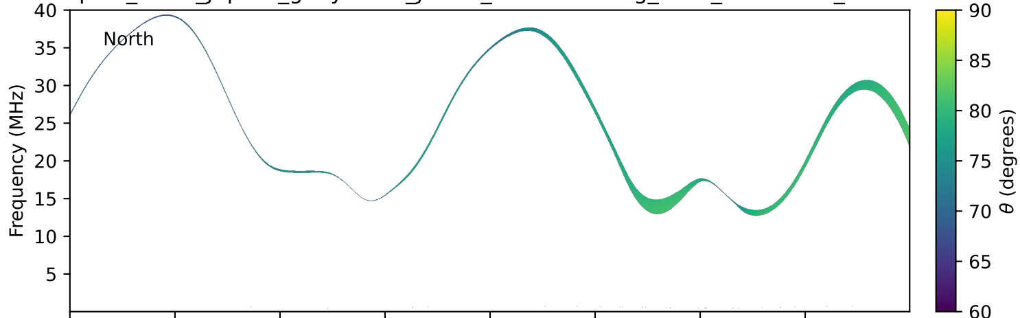
expres_earth_jupiter_ganymede_jrm33_lossc-wid1deg_3kev_20270828_v11.cdf
