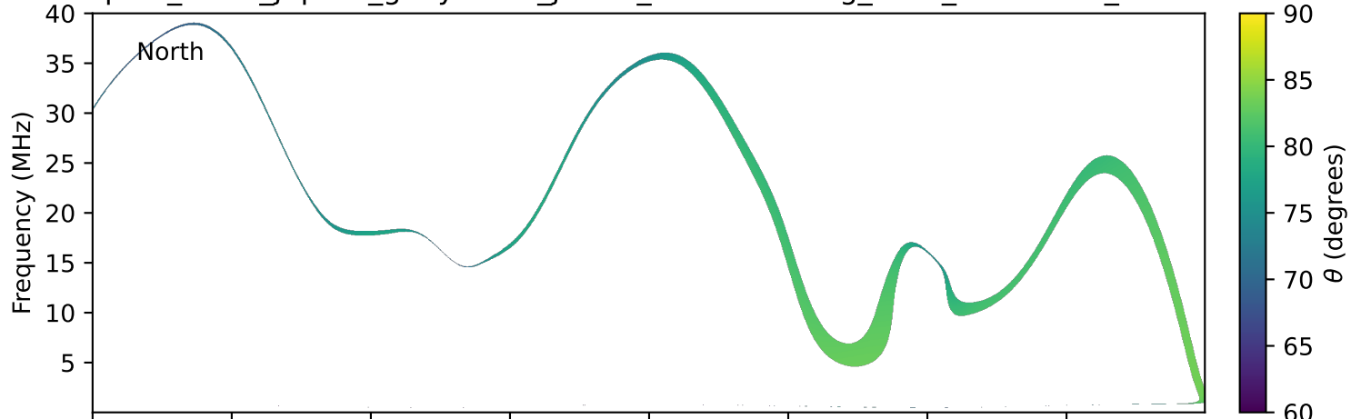
expres_earth_jupiter_ganymede_jrm33_lossc-wid1deg_3kev_20270821_v11.cdf
