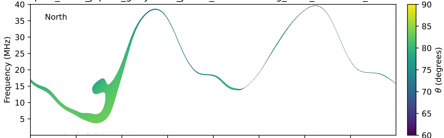
expres_earth_jupiter_ganymede_jrm33_lossc-wid1deg_3kev_20270819_v11.cdf
