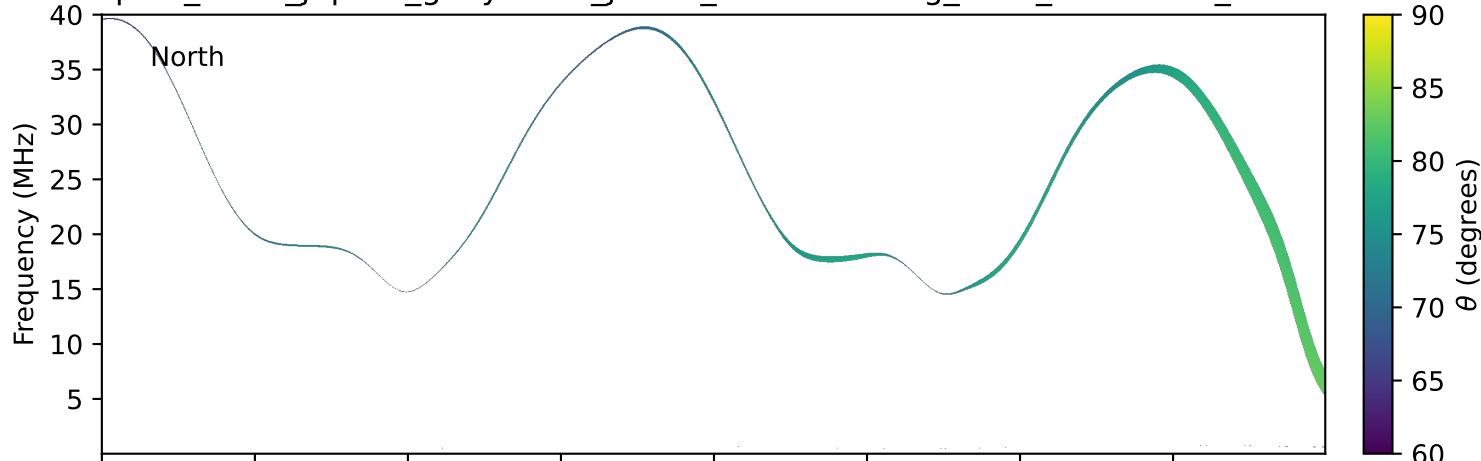
expres_earth_jupiter_ganymede_jrm33_lossc-wid1deg_3kev_20270807_v11.cdf
