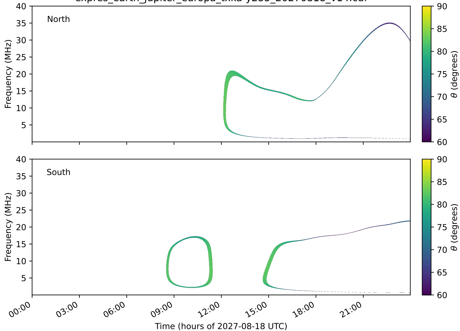
expres_earth_jupiter_europa_txka-y235_20270818_v14.cdf
