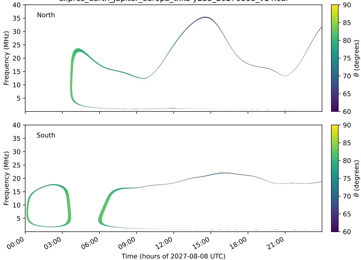
expres_earth_jupiter_europa_txka-y235_20270808_v14.cdf
