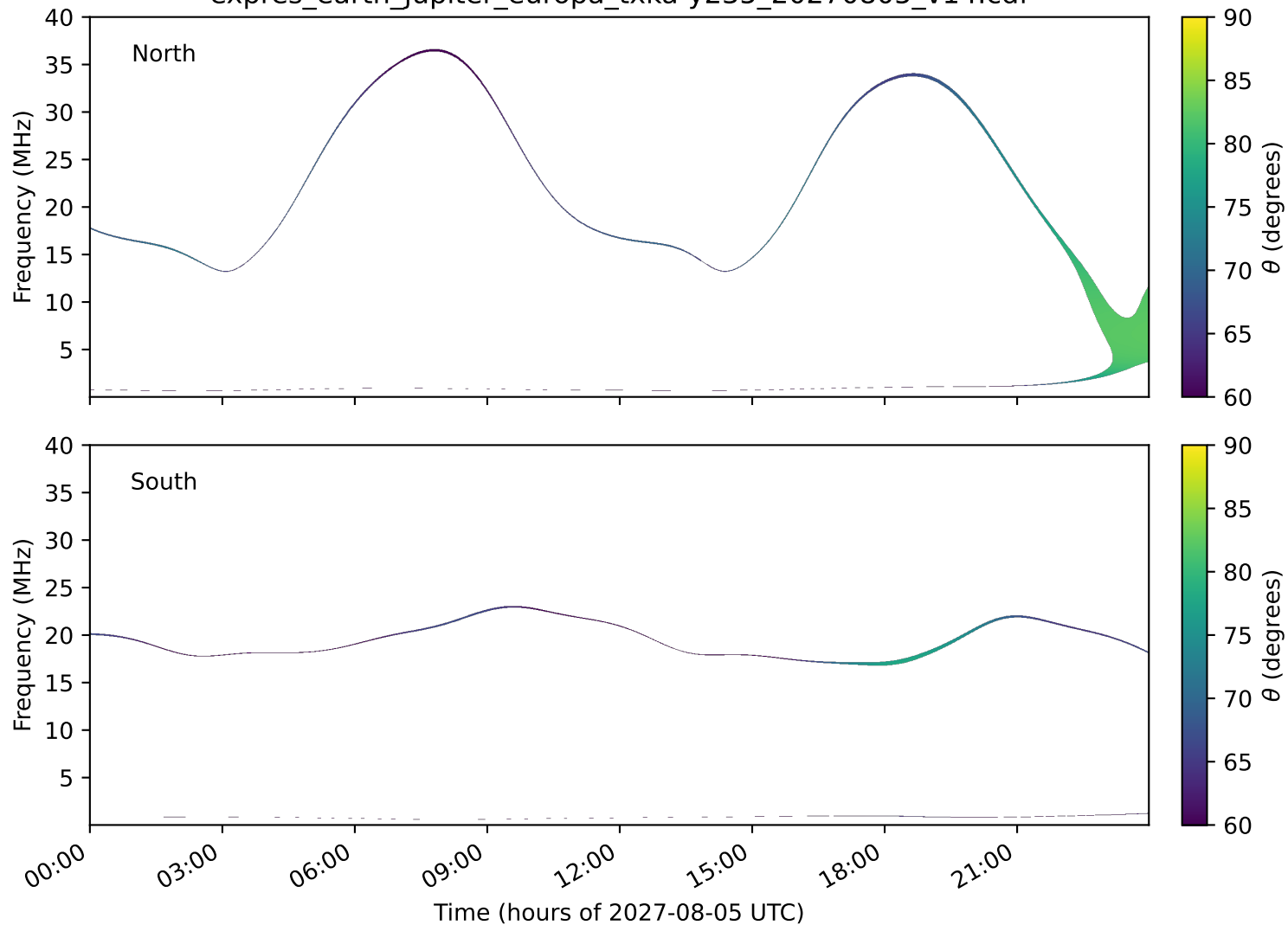
expres_earth_jupiter_europa_txka-y235_20270805_v14.cdf
