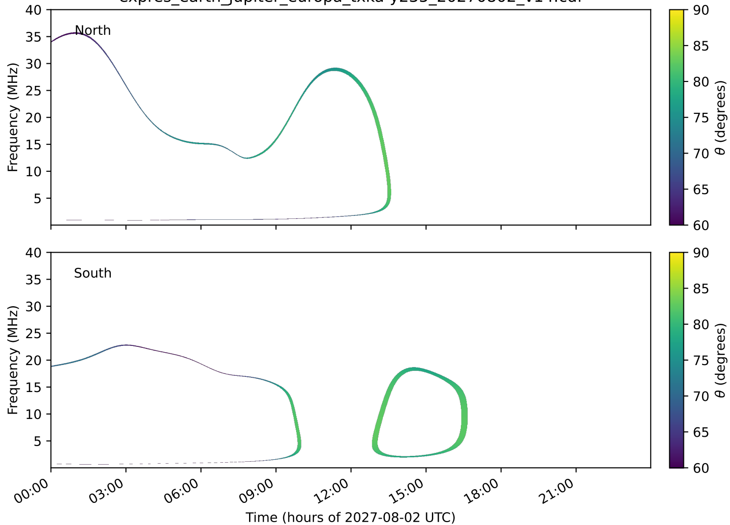
expres_earth_jupiter_europa_txka-y235_20270802_v14.cdf
