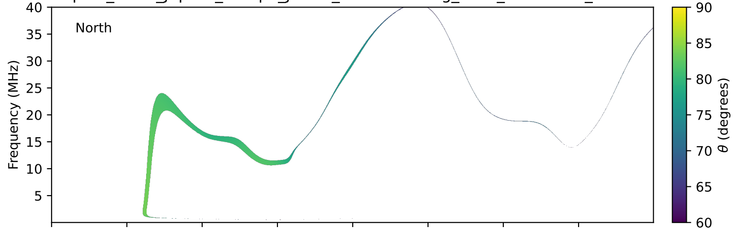
expres_earth_jupiter_europa_jrm33_lossc-wid1deg_3kev_20270808_v11.cdf
