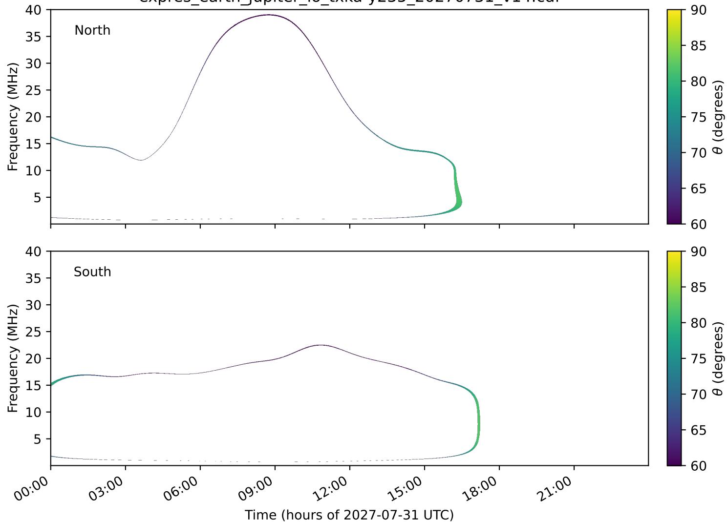
expres_earth_jupiter_io_txka-y235_20270731_v14.cdf
