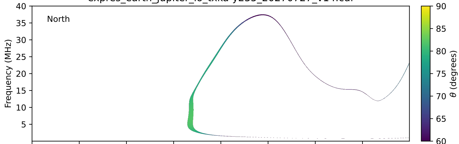
expres_earth_jupiter_io_txka-y235_20270727_v14.cdf
