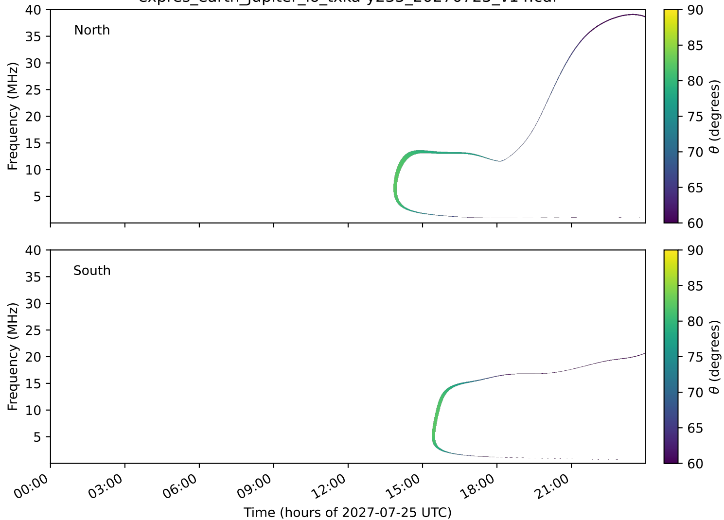
expres_earth_jupiter_io_txka-y235_20270725_v14.cdf
