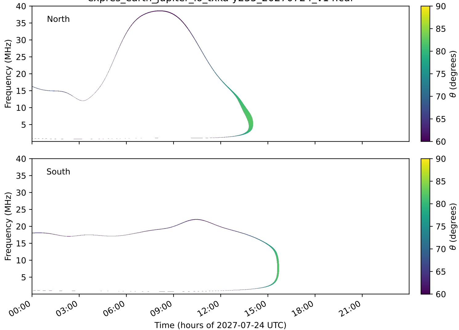
expres_earth_jupiter_io_txka-y235_20270724_v14.cdf
