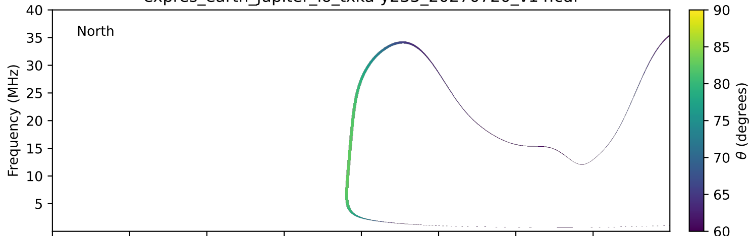
expres_earth_jupiter_io_txka-y235_20270720_v14.cdf
