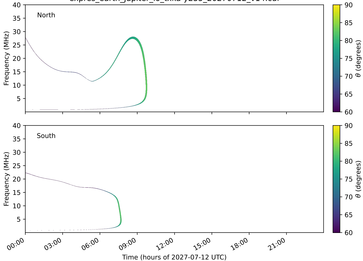
expres_earth_jupiter_io_txka-y235_20270712_v14.cdf
