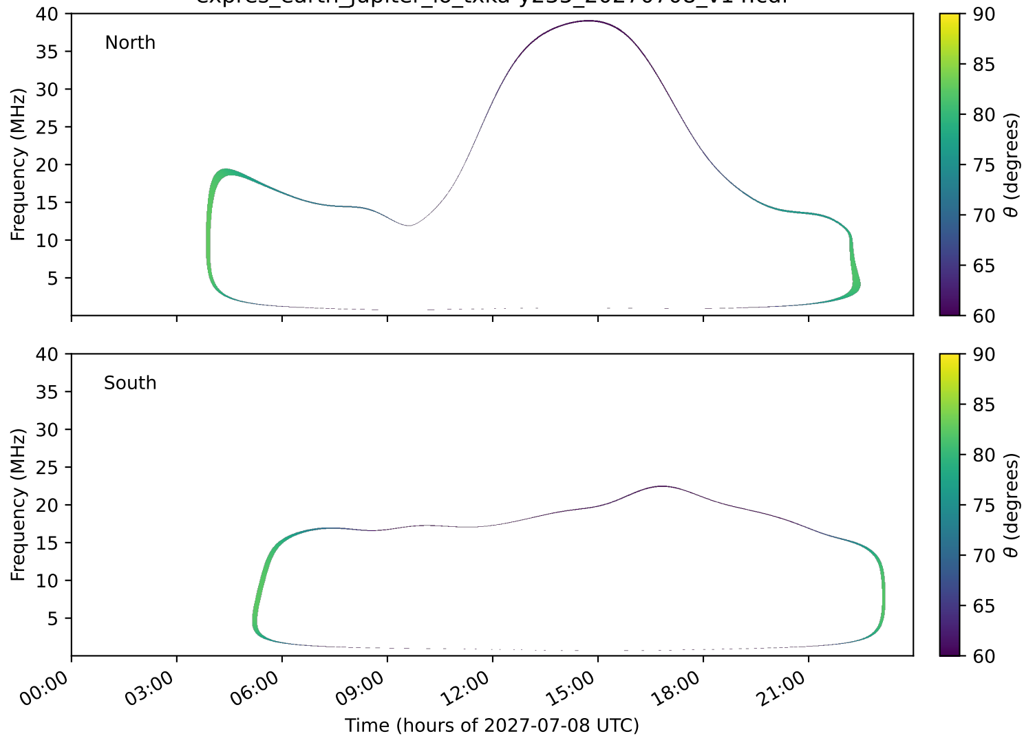
expres_earth_jupiter_io_txka-y235_20270708_v14.cdf
