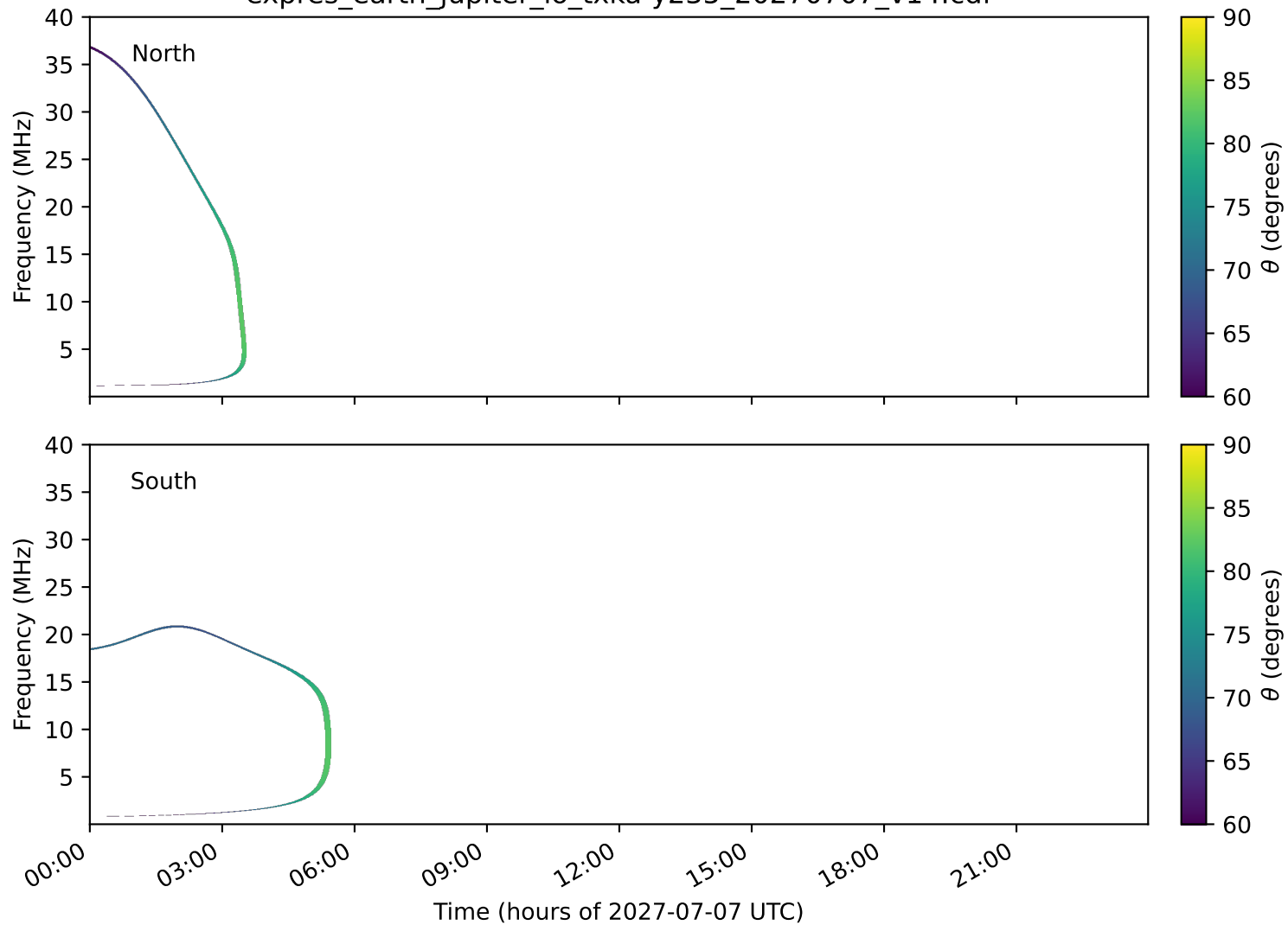
expres_earth_jupiter_io_txka-y235_20270707_v14.cdf
