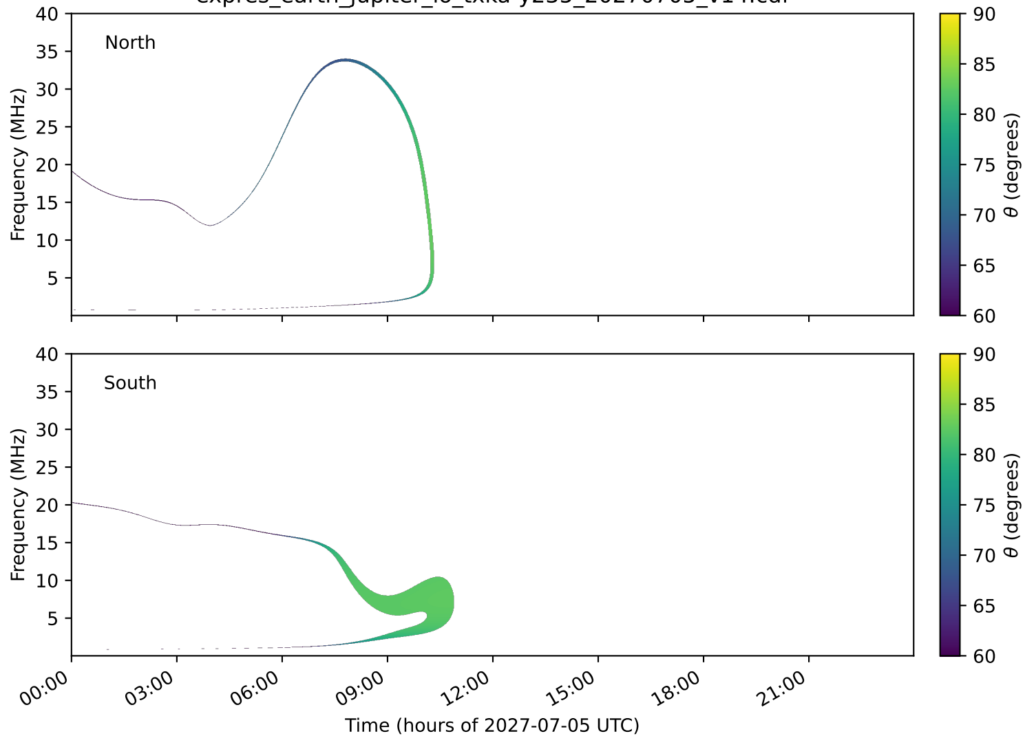
expres_earth_jupiter_io_txka-y235_20270705_v14.cdf
