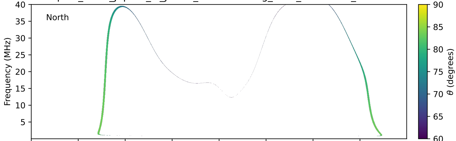
expres_earth_jupiter_io_jrm33_lossc-wid1deg_3kev_20270729_v11.cdf
