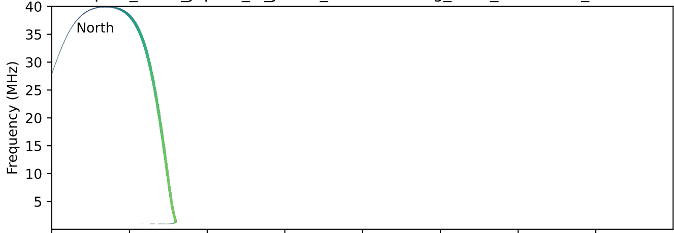
expres_earth_jupiter_io_jrm33_lossc-wid1deg_3kev_20270728_v11.cdf
