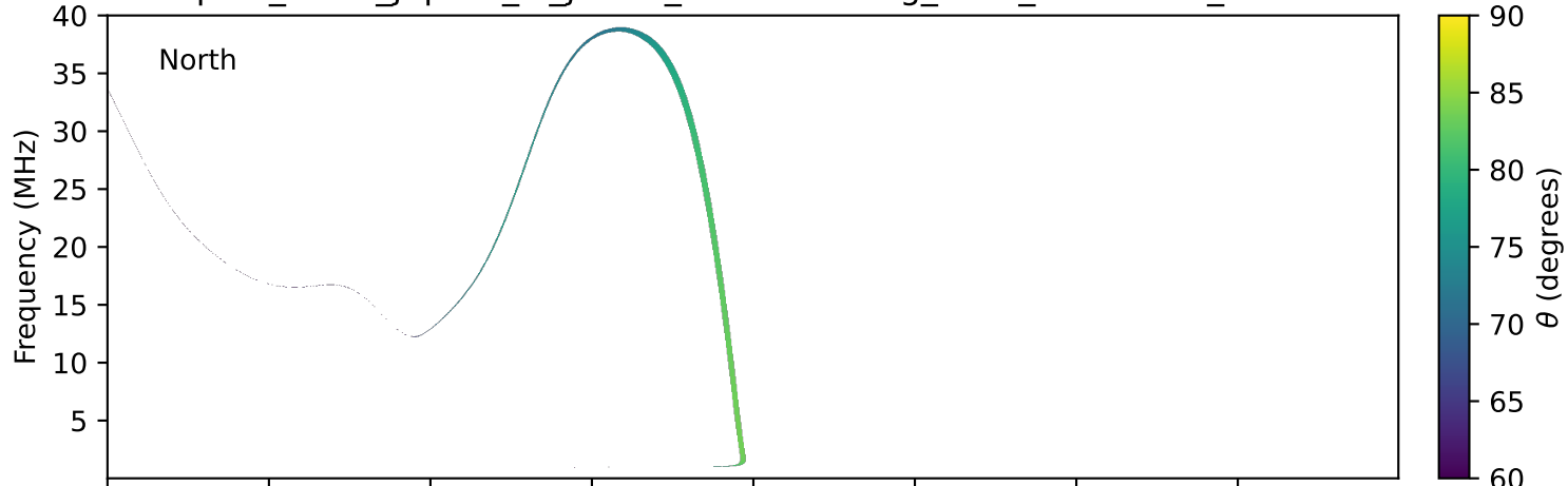
expres_earth_jupiter_io_jrm33_lossc-wid1deg_3kev_20270719_v11.cdf
