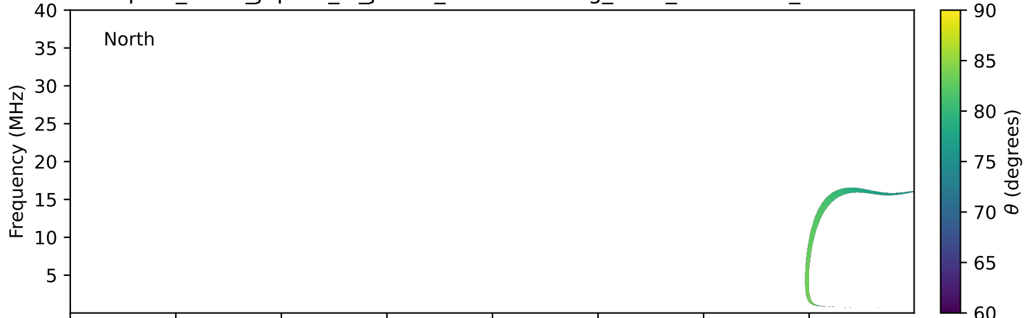
expres_earth_jupiter_io_jrm33_lossc-wid1deg_3kev_20270716_v11.cdf
