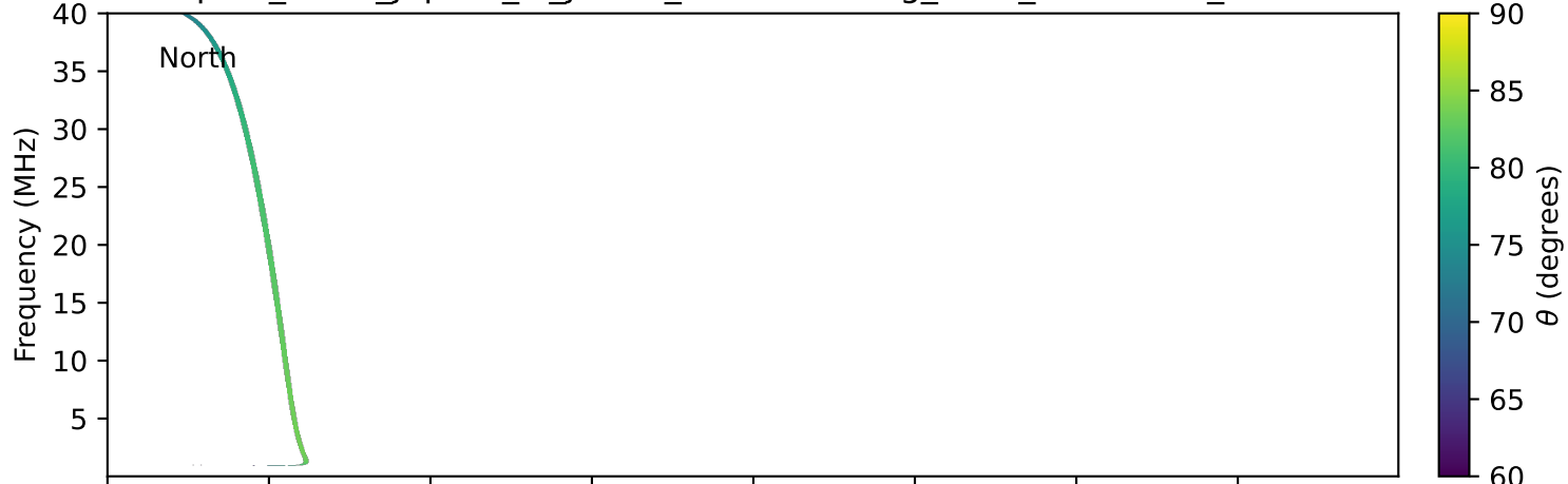
expres_earth_jupiter_io_jrm33_lossc-wid1deg_3kev_20270714_v11.cdf
