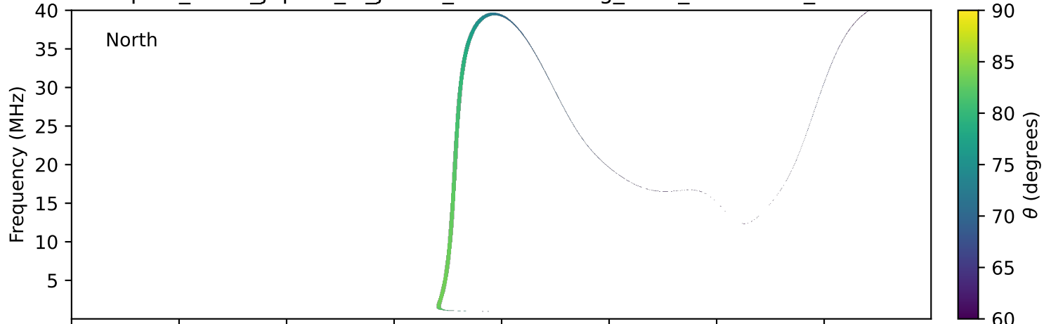
expres_earth_jupiter_io_jrm33_lossc-wid1deg_3kev_20270706_v11.cdf
