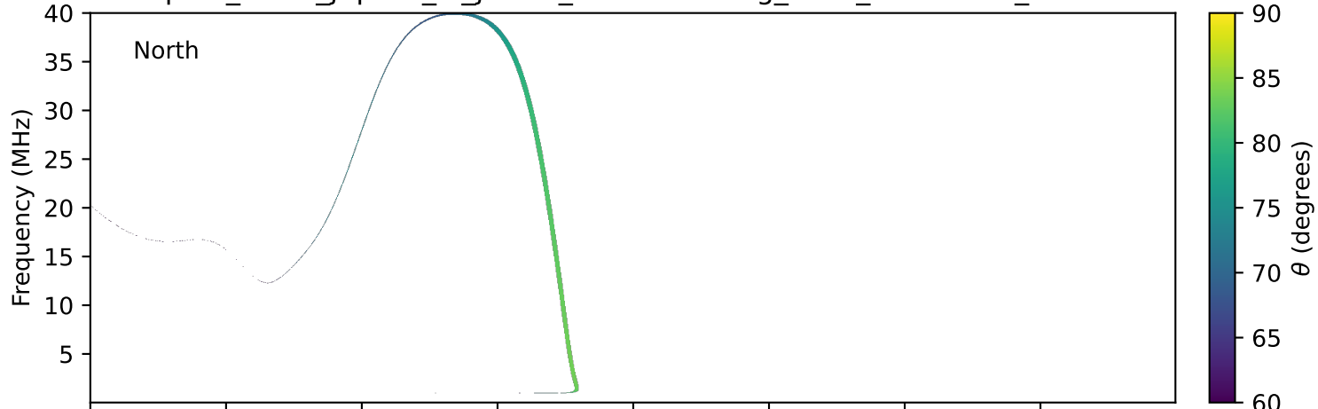
expres_earth_jupiter_io_jrm33_lossc-wid1deg_3kev_20270705_v11.cdf
