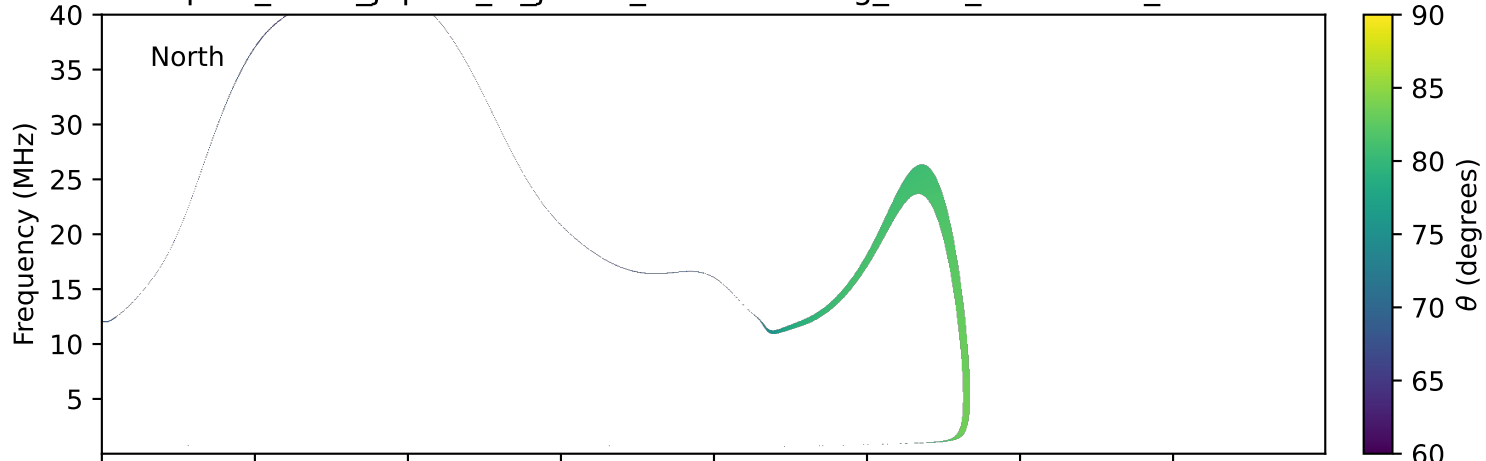
expres_earth_jupiter_io_jrm33_lossc-wid1deg_3kev_20270703_v11.cdf
