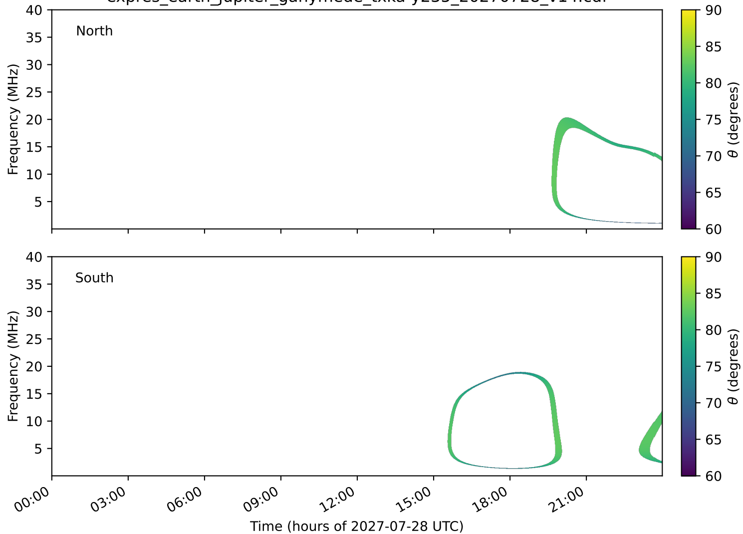
expres_earth_jupiter_ganymede_txka-y235_20270728_v14.cdf
