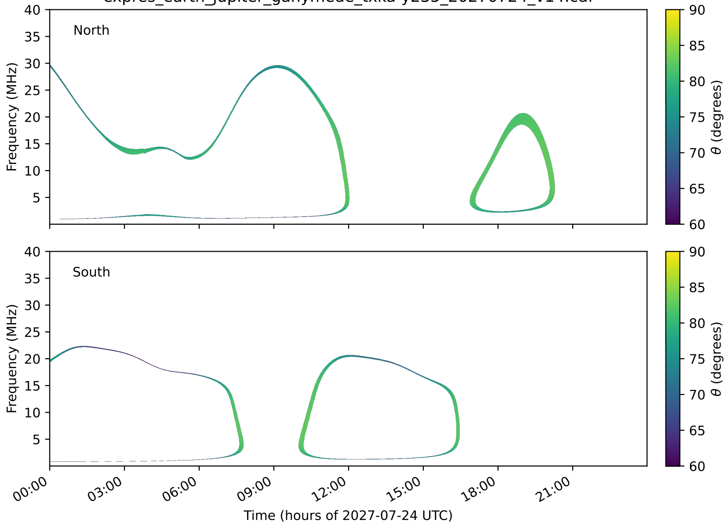
expres_earth_jupiter_ganymede_txka-y235_20270724_v14.cdf
