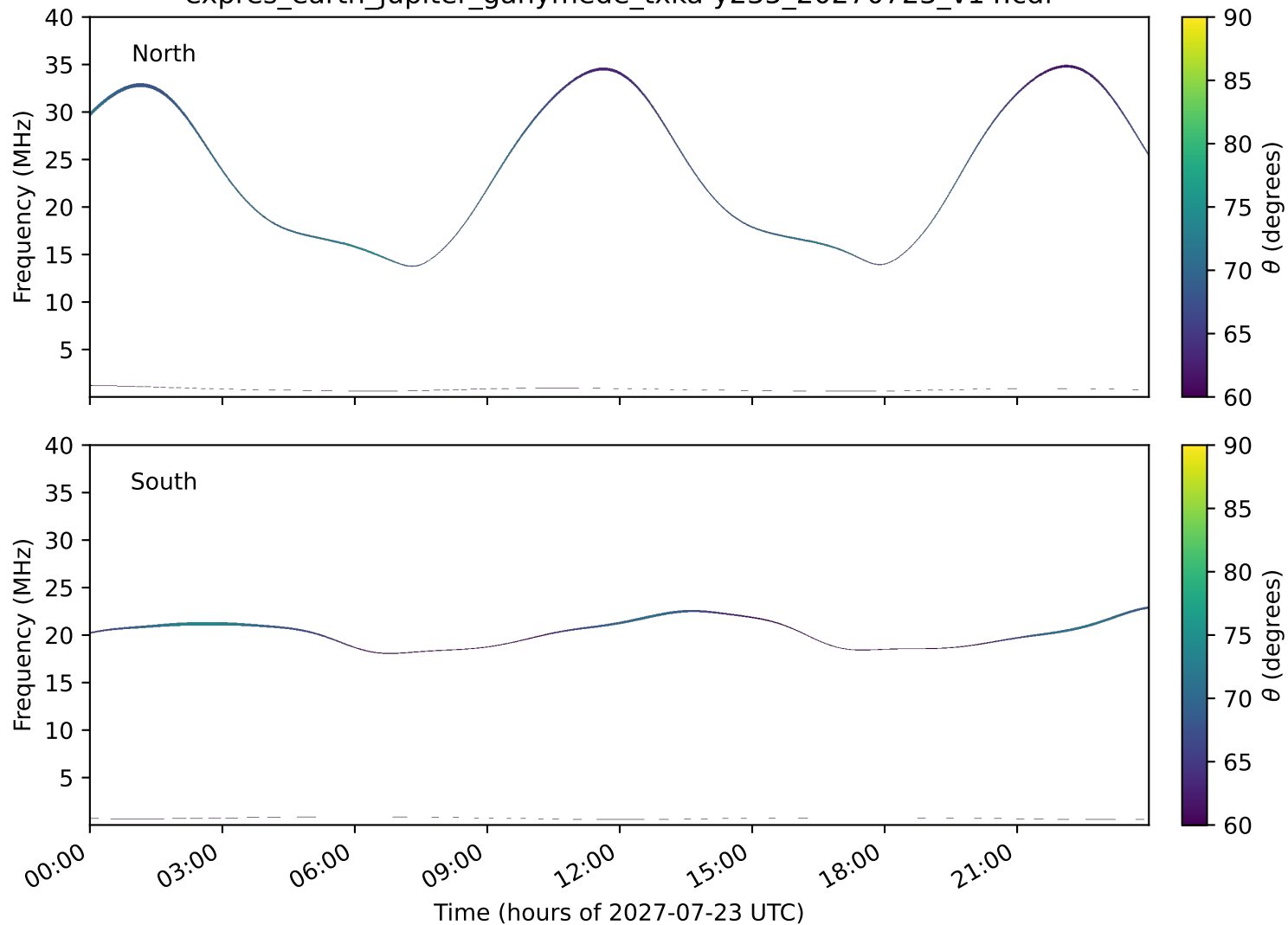
expres_earth_jupiter_ganymede_txka-y235_20270723_v14.cdf
