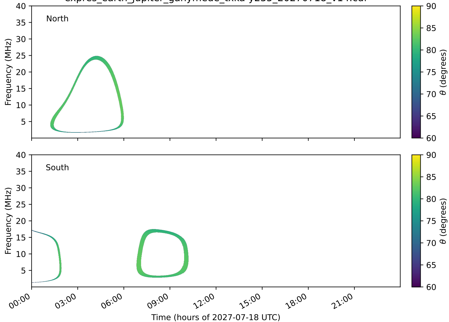
expres_earth_jupiter_ganymede_txka-y235_20270718_v14.cdf
