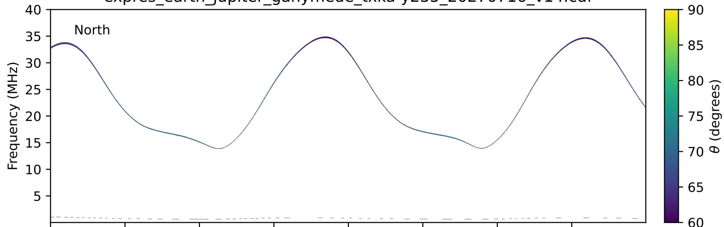
expres_earth_jupiter_ganymede_txka-y235_20270716_v14.cdf
