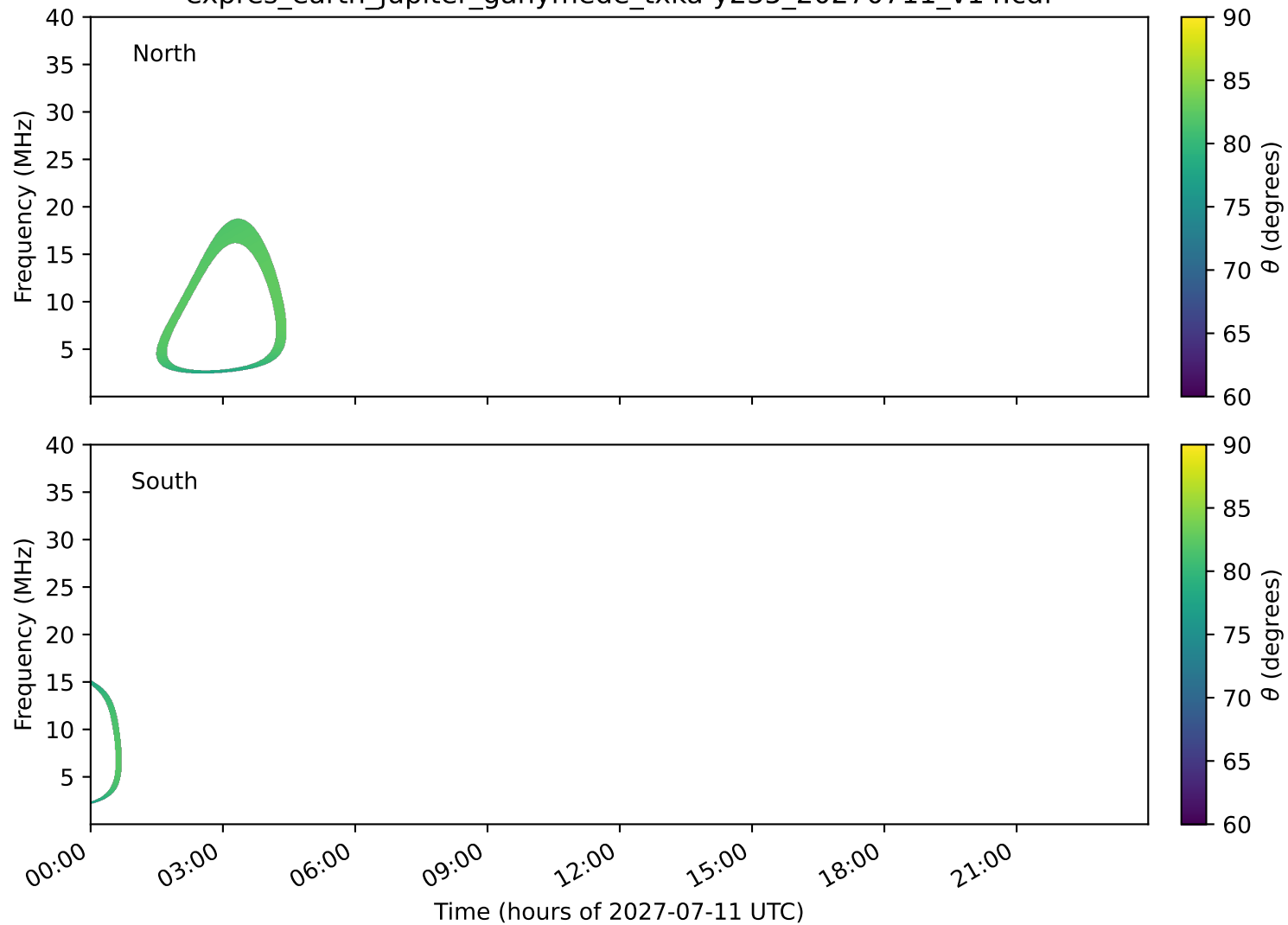
expres_earth_jupiter_ganymede_txka-y235_20270711_v14.cdf
