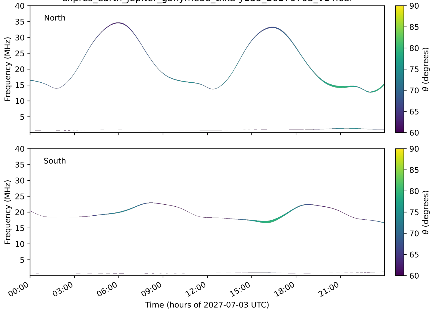
expres_earth_jupiter_ganymede_txka-y235_20270703_v14.cdf
