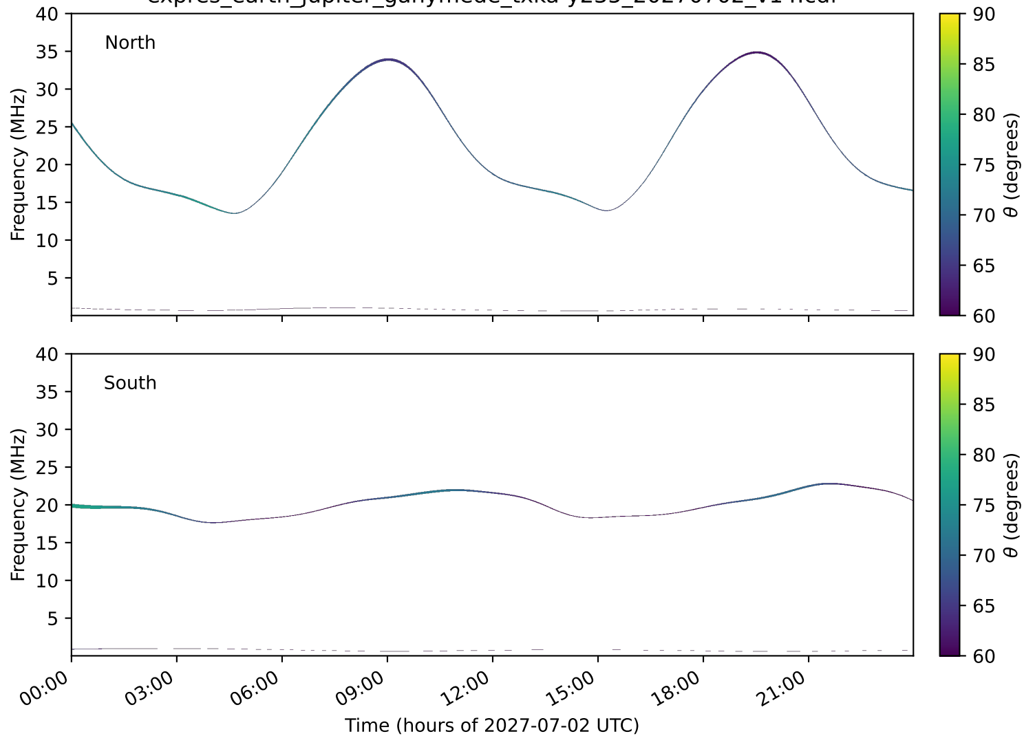
expres_earth_jupiter_ganymede_txka-y235_20270702_v14.cdf
