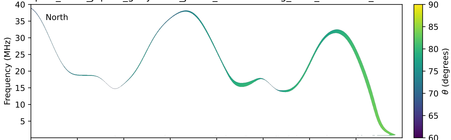
expres_earth_jupiter_ganymede_jrm33_lossc-wid1deg_3kev_20270731_v11.cdf
