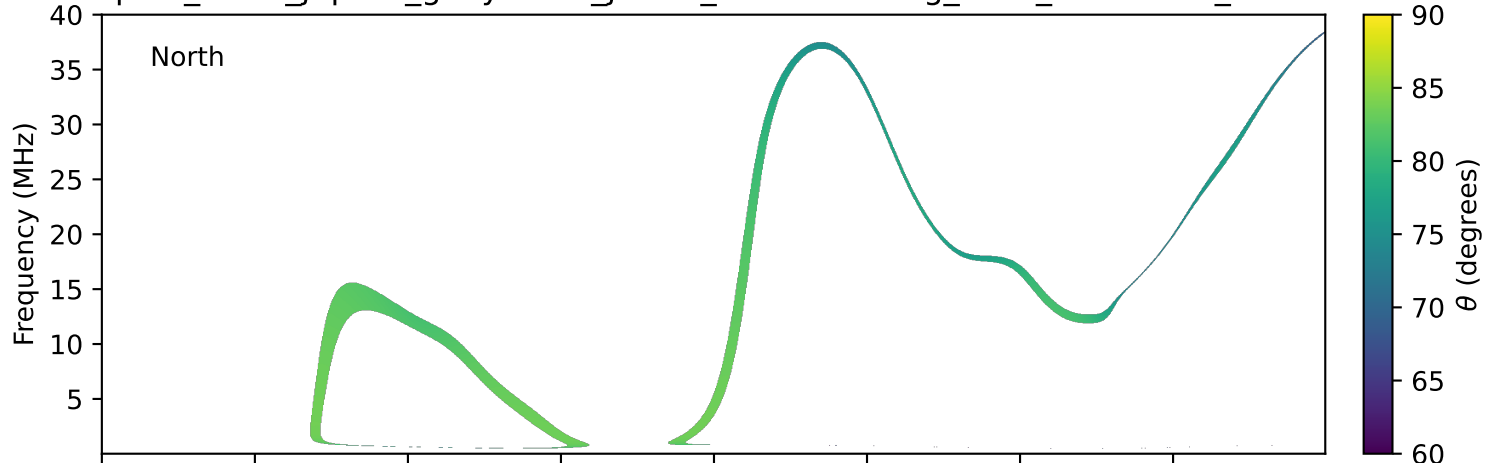
expres_earth_jupiter_ganymede_jrm33_lossc-wid1deg_3kev_20270715_v11.cdf
