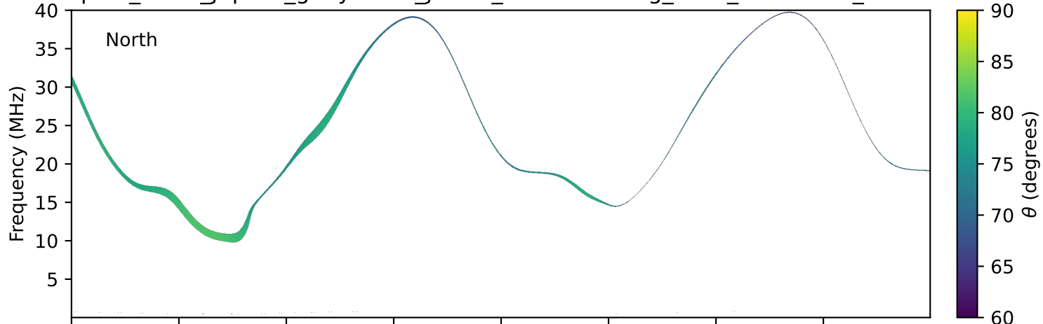
expres_earth_jupiter_ganymede_jrm33_lossc-wid1deg_3kev_20270709_v11.cdf
