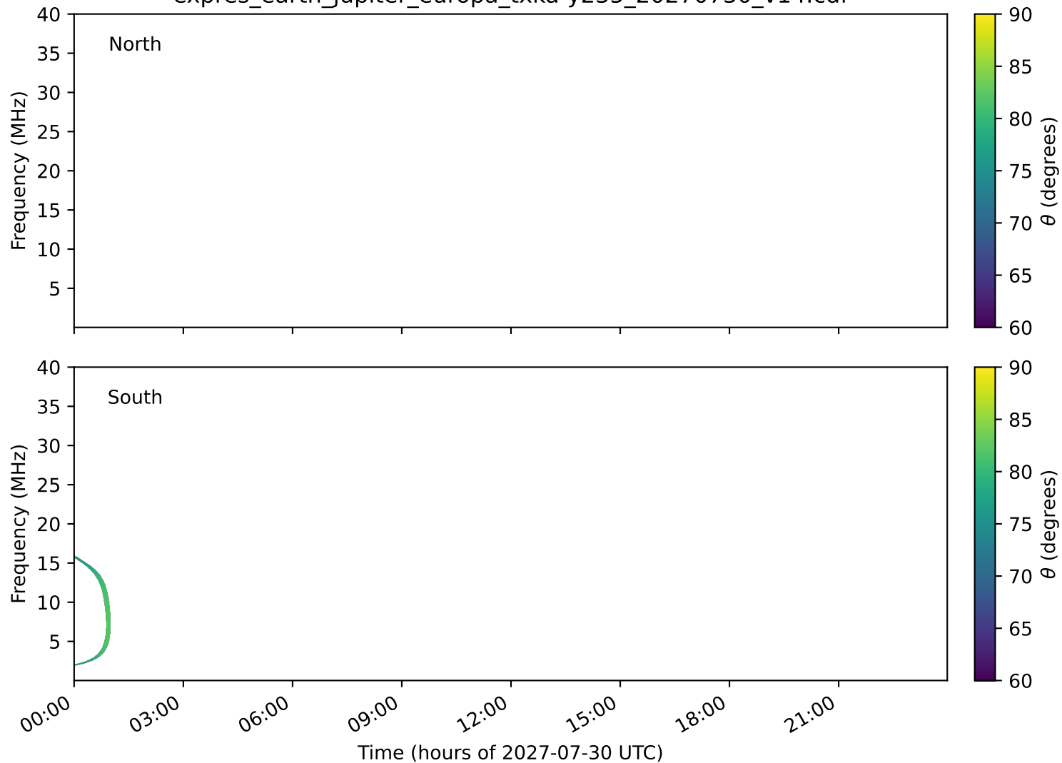
expres_earth_jupiter_europa_txka-y235_20270730_v14.cdf
