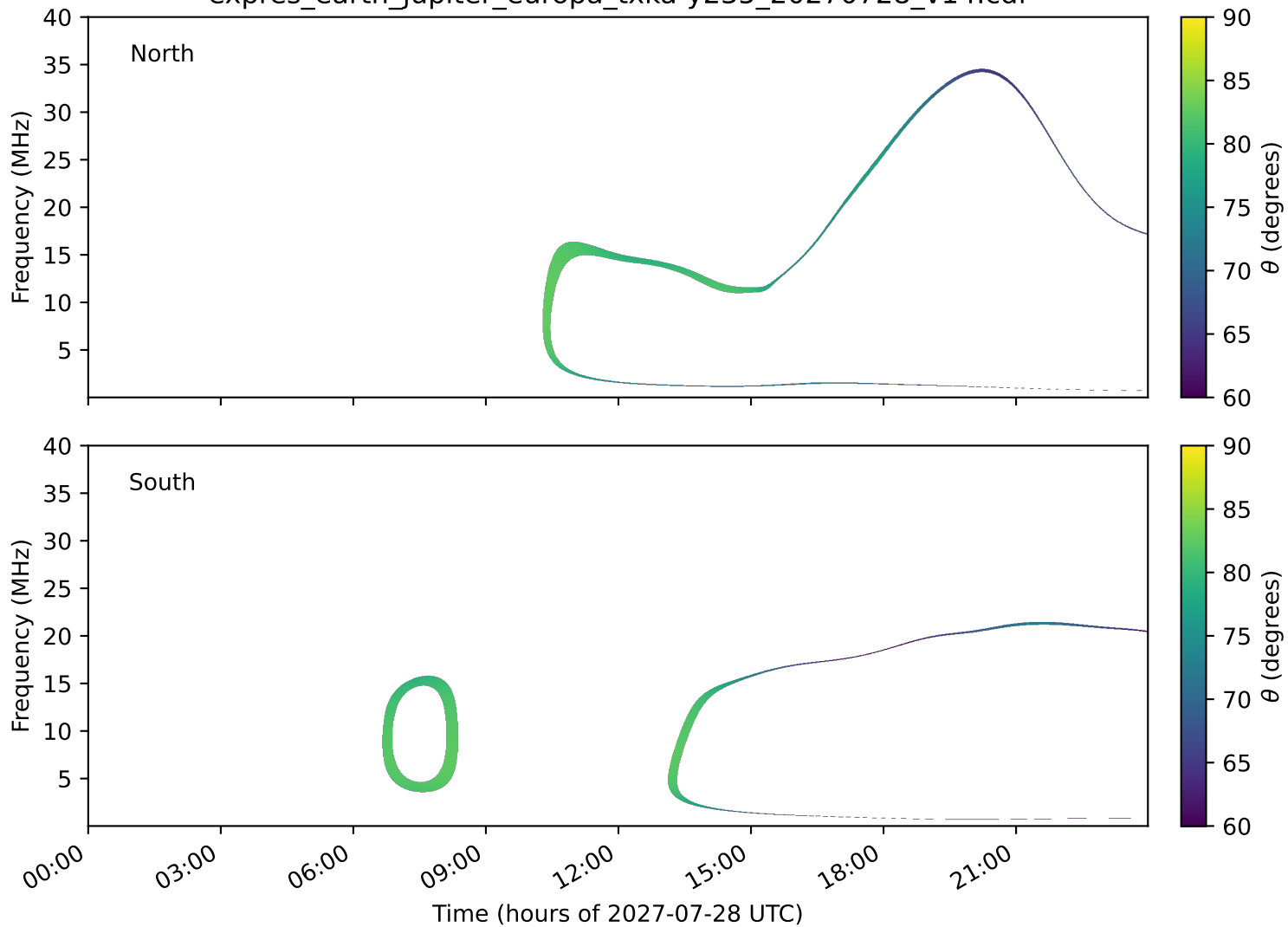
expres_earth_jupiter_europa_txka-y235_20270728_v14.cdf
