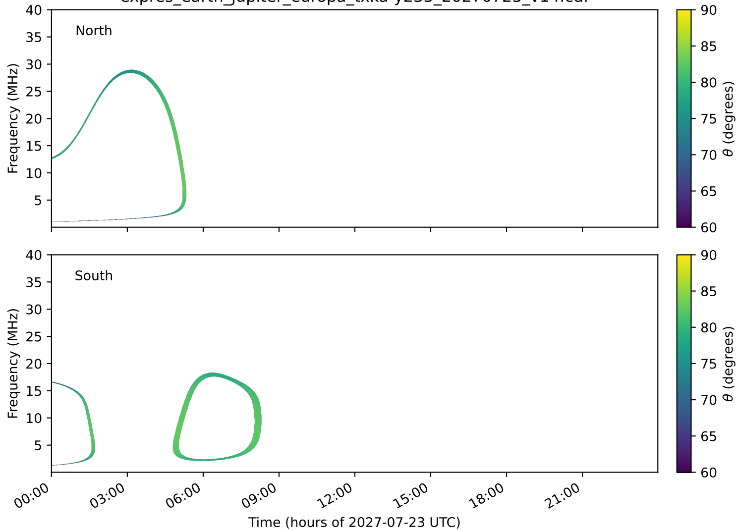
expres_earth_jupiter_europa_txka-y235_20270723_v14.cdf
