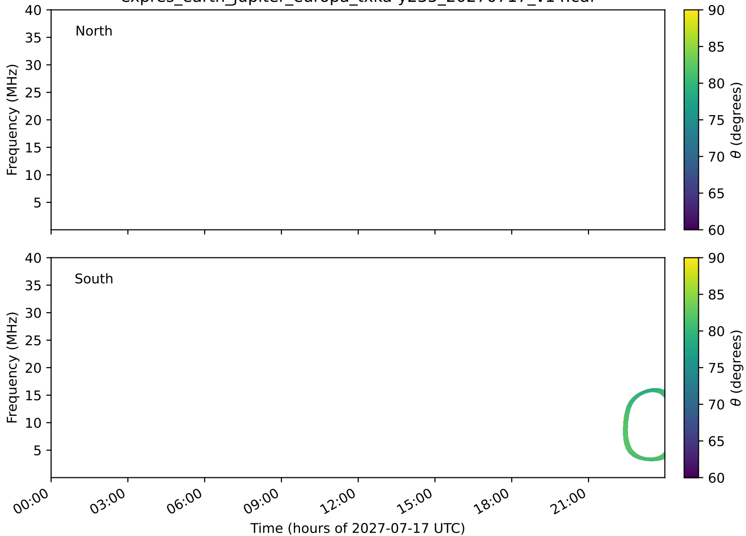
expres_earth_jupiter_europa_txka-y235_20270717_v14.cdf
