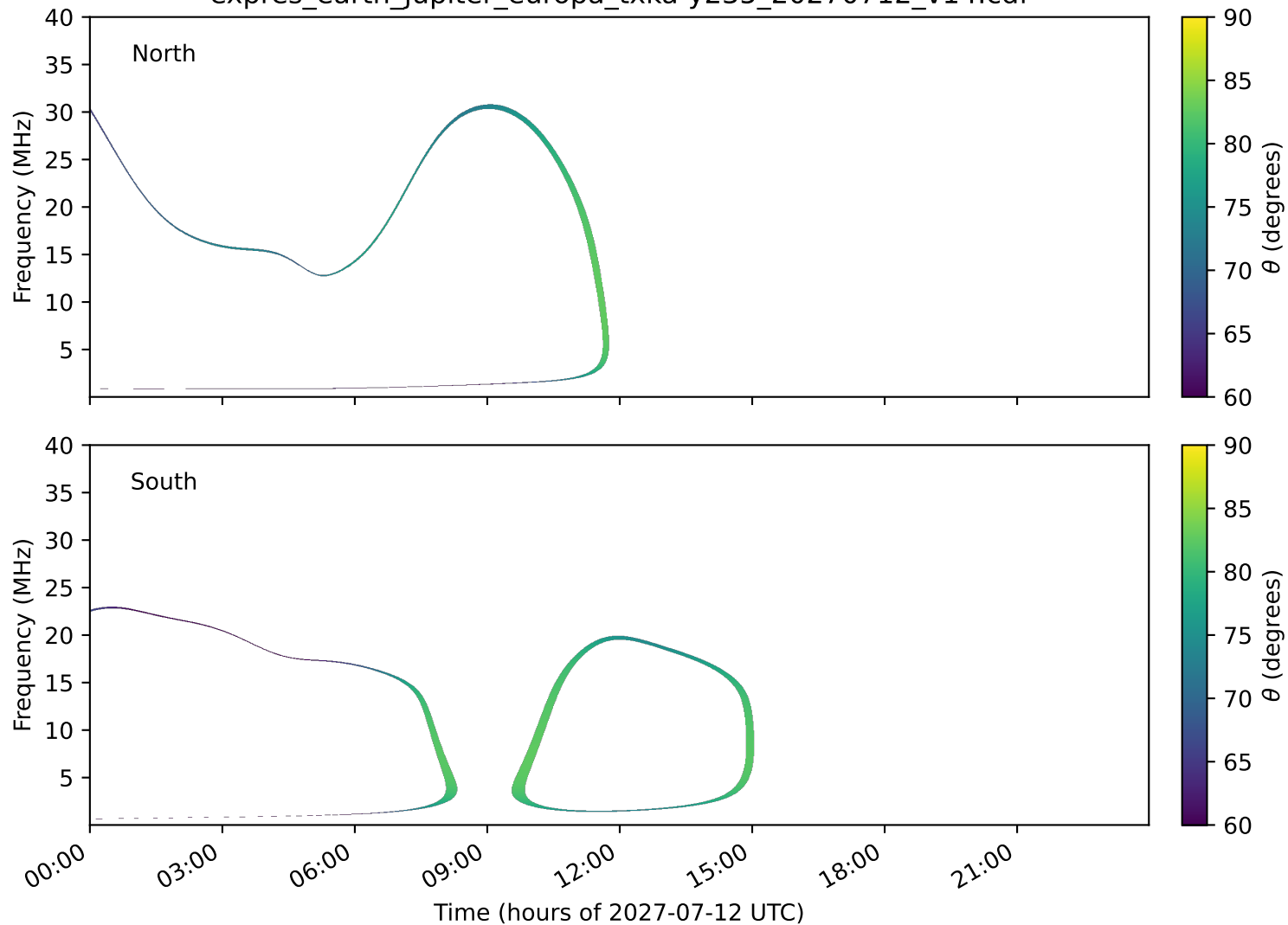
expres_earth_jupiter_europa_txka-y235_20270712_v14.cdf
