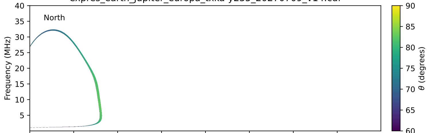
expres_earth_jupiter_europa_txka-y235_20270709_v14.cdf
