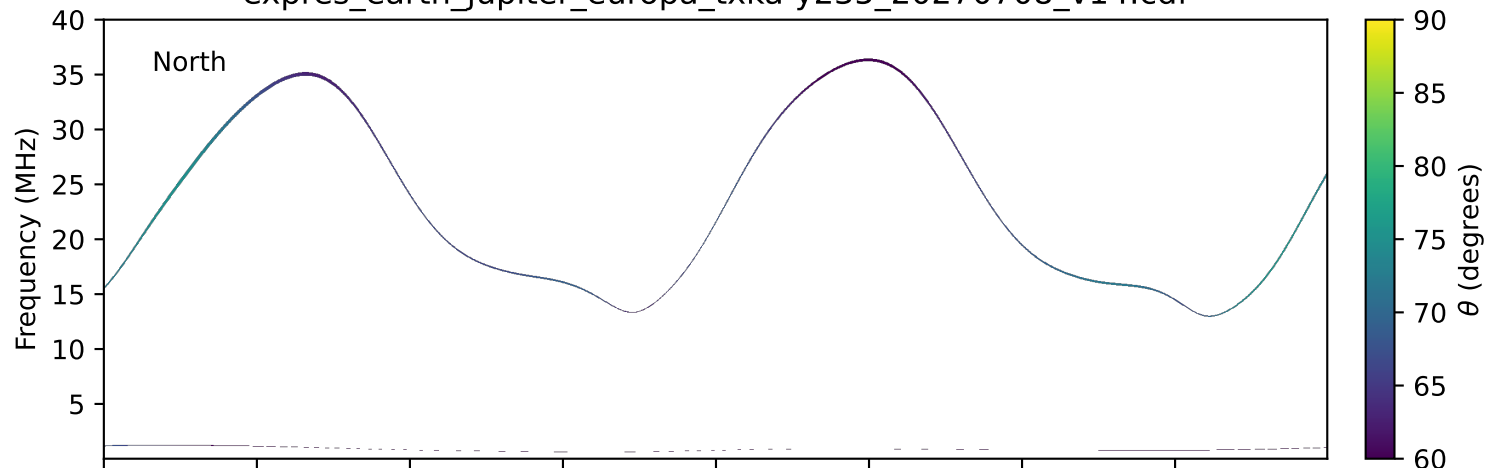
expres_earth_jupiter_europa_txka-y235_20270708_v14.cdf
