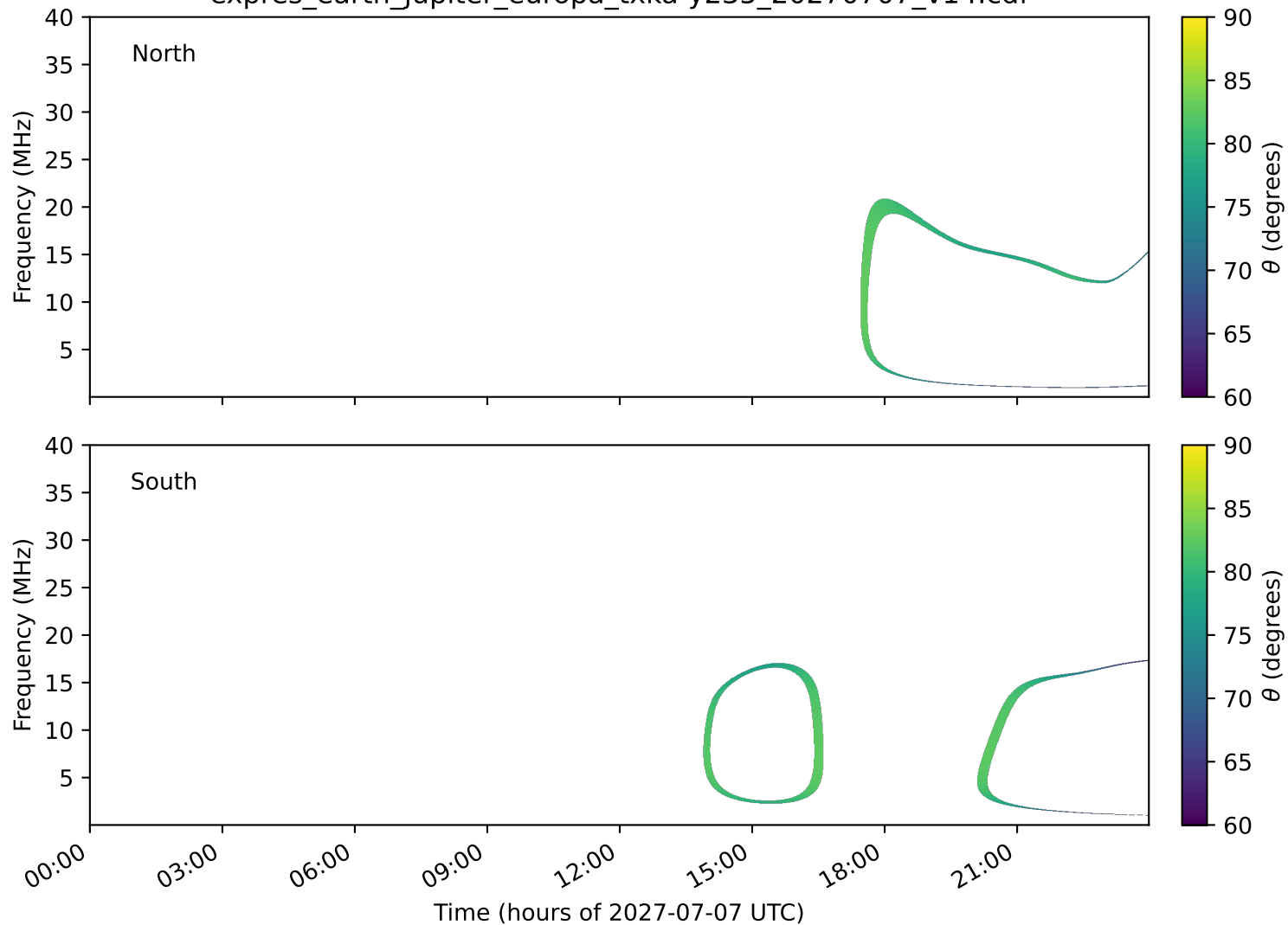
expres_earth_jupiter_europa_txka-y235_20270707_v14.cdf
