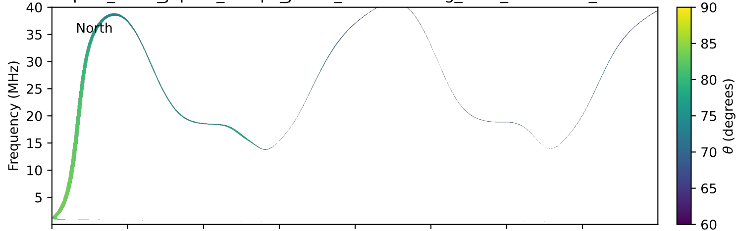
expres_earth_jupiter_europa_jrm33_lossc-wid1deg_3kev_20270725_v11.cdf
