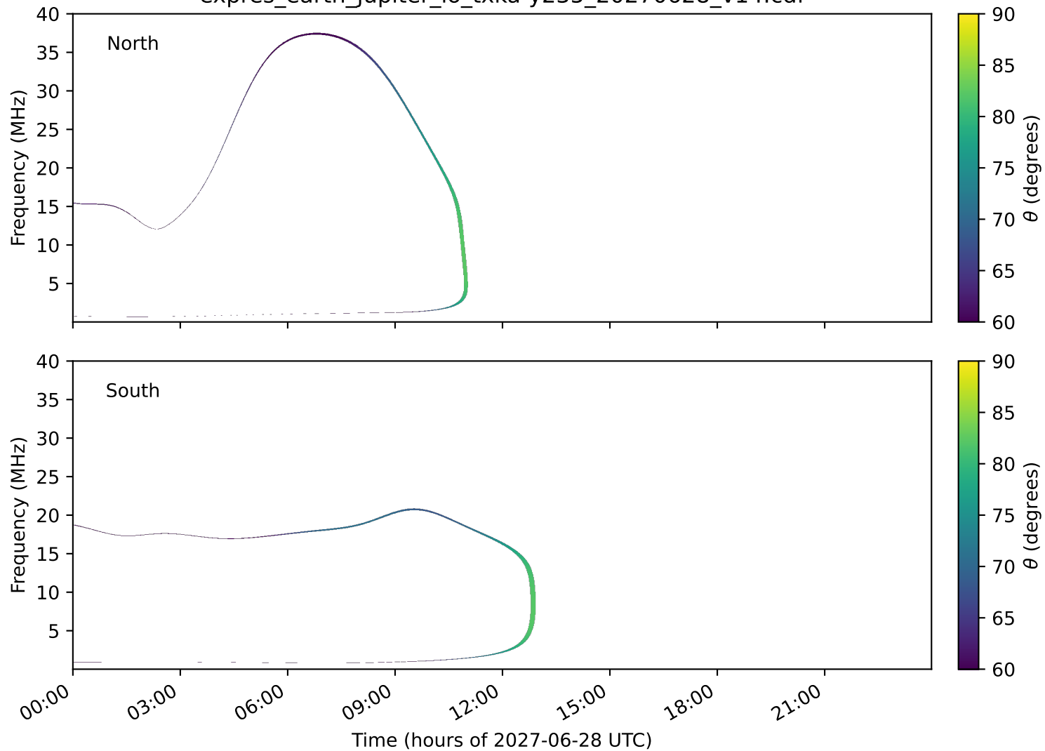
expres_earth_jupiter_io_txka-y235_20270628_v14.cdf
