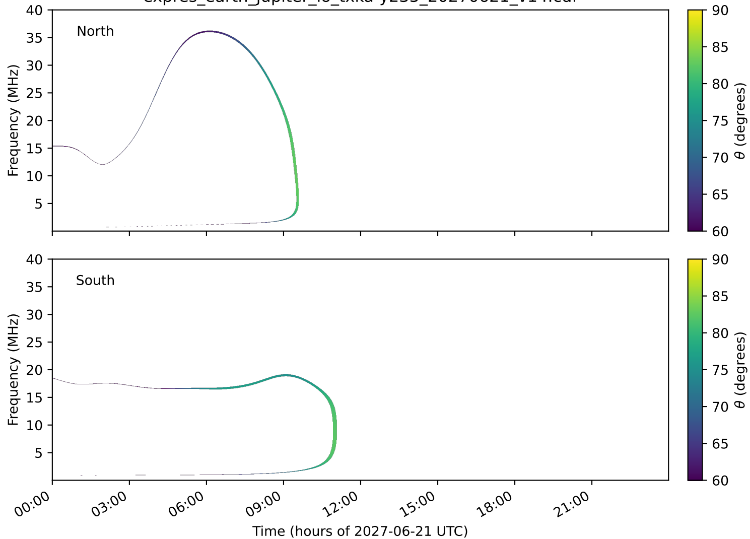
expres_earth_jupiter_io_txka-y235_20270621_v14.cdf
